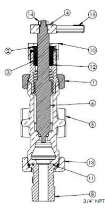
LOWER VALVE
