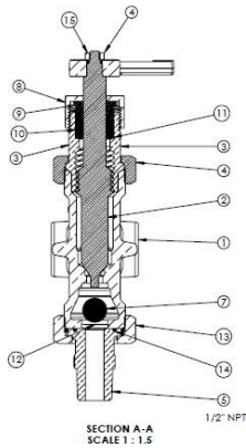
UPPER VALVE
