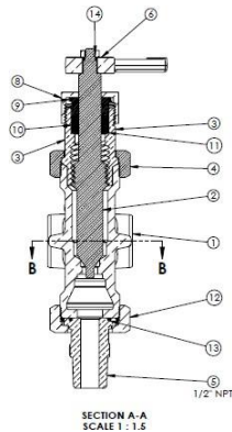
LOWER VALVE
