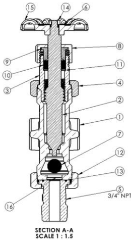
UPPER VALVE
