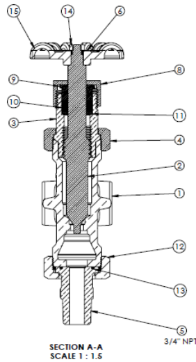
LOWER VALVE
